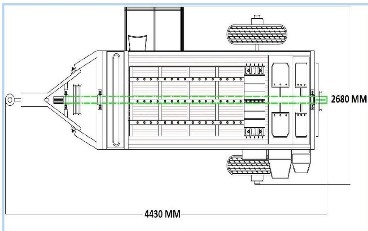
Top view of Paddy Thresher
